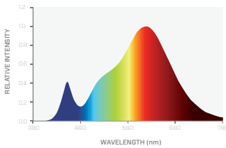
SPECTRAL POWER DISTRIBUTION - 3000K (830)
