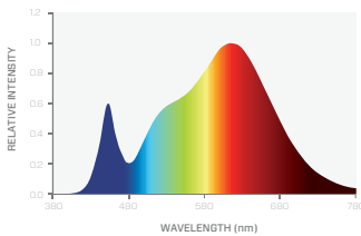
SPECTRAL POWER DISTRIBUTION - 4000K (840)
